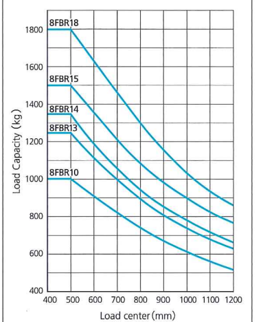
Load Capacity Charts
